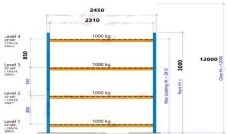
FRONT VIEW (A)
